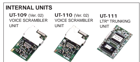
INTERNAL UNITS UT-109 (Ver. 02) VOICE SCRAMBLER UNIT : Non-rolling type voice scrambler. UT-110 (Ver. 02) VOICE SCRAMBLER UNIT : Rolling type voice scrambler. UT-111 LTR® TRUNKING UNIT : Provides LTR® trunking capabilities.
